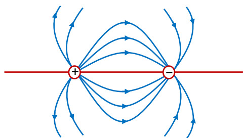
ELOF due to equal positive and negative charges
