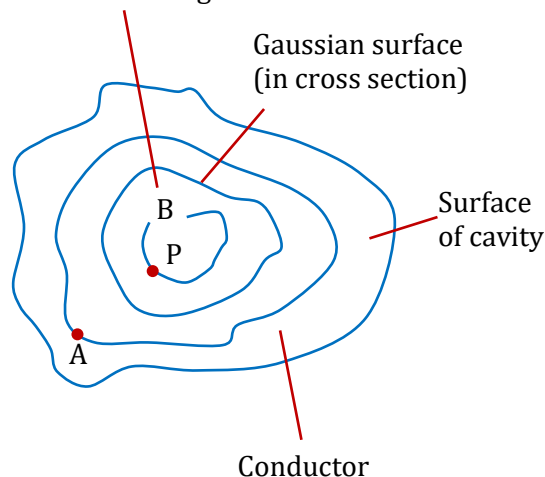
Cross section of equipotential surface through P
