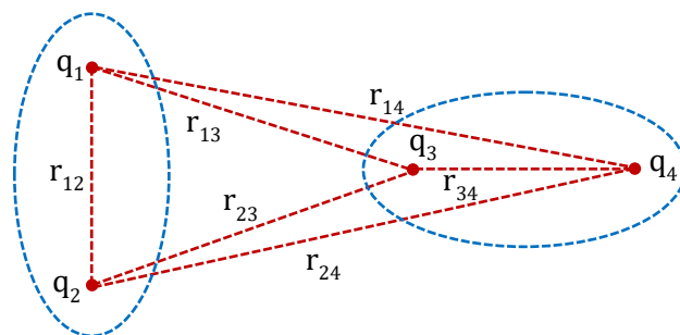
System A = q_1 + q_2
