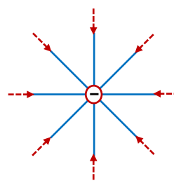
ELOF of Isolated negative charge
